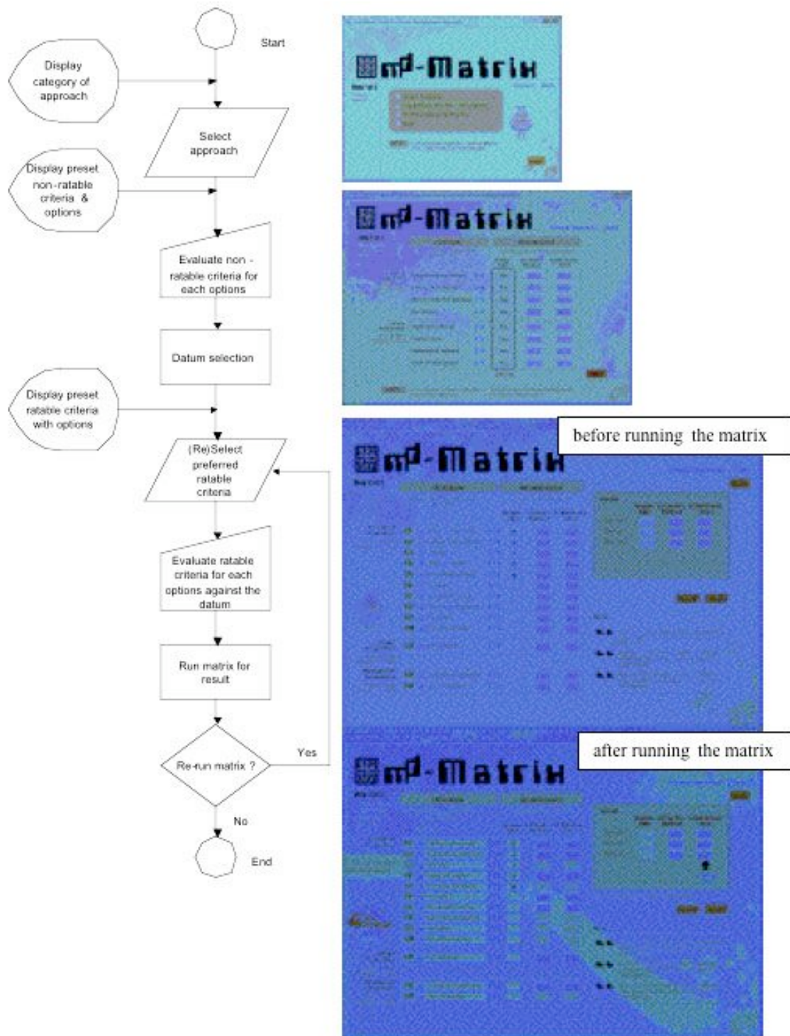
Figure 1: Flowchart and screen designs of m d -Matrix
