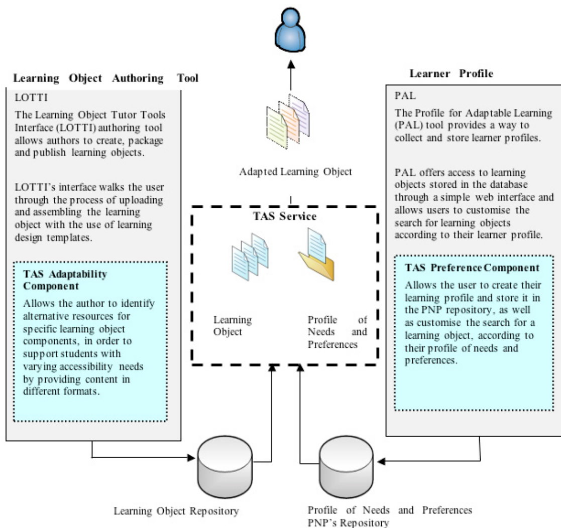
Figure 2: The TASS model
